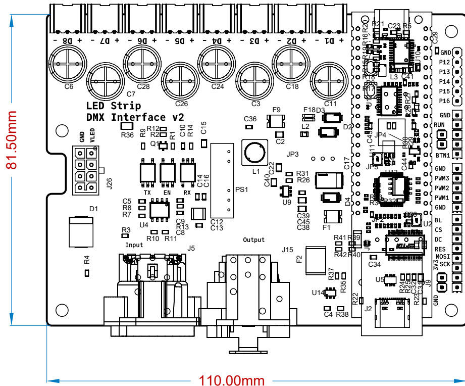
Top side component view (Scale 1:1)
